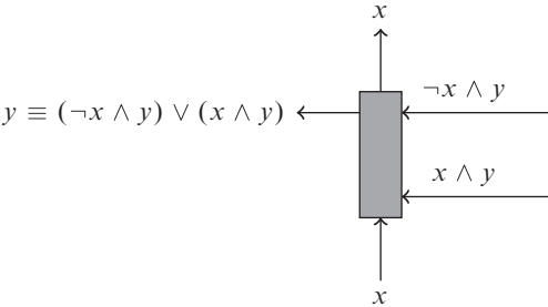
Figure 6.19 Switch gate with inputs and outputs interchanged.
