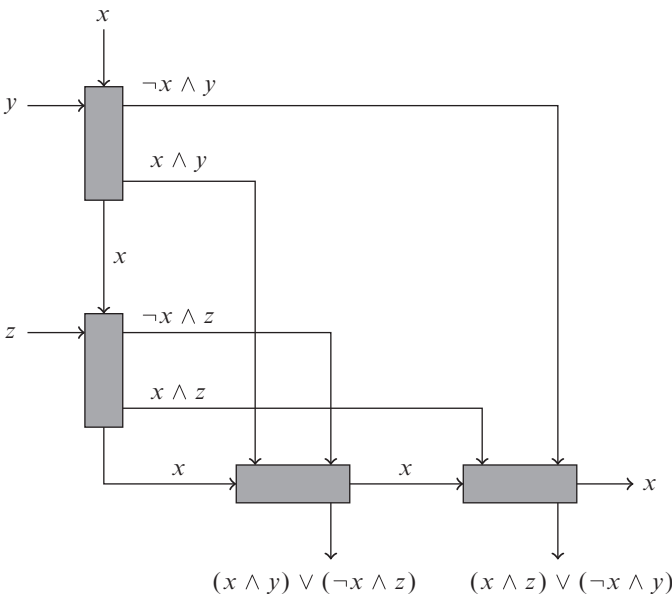
Figure 6.20 Fredkin gate constructed from switch gates.
