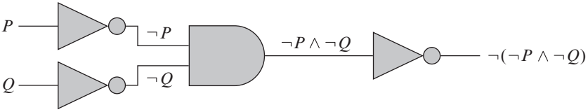
Figure 6.6 A circuit for \neg(\neg P \wedge \neg Q) .
