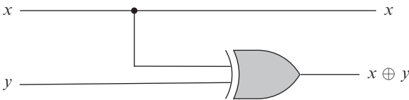
Figure 6.12 A circuit for CNOT .
