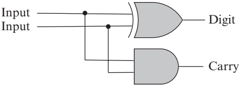
Figure 6.10 A half-adder circuit.
