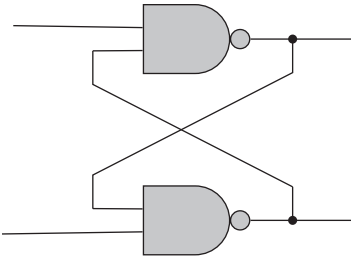
Figure 6.11 A flip-flop using two NAND gates.
