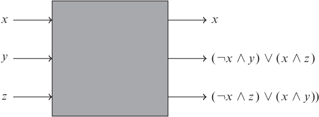
Figure 6.22 Billiard-ball Fredkin gate to be used in circuits.
