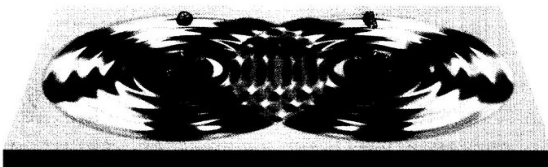
Superposition of waves: If two stones are dropped in a pond close to each other the ripples will spread out and meet, forming a superposition that has a pattern very different to the two sets of concentric waves, due to interference.
